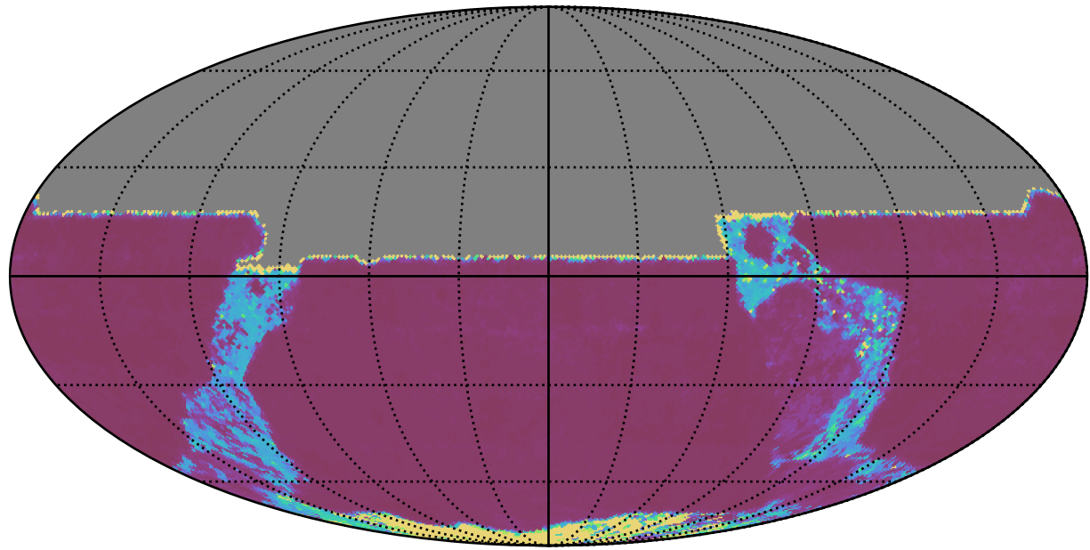
ddf_acor_sf30_lsf40_lsr50_v3.4_10yrs All sky y band: 20thPercentile Inter-Night Gap
