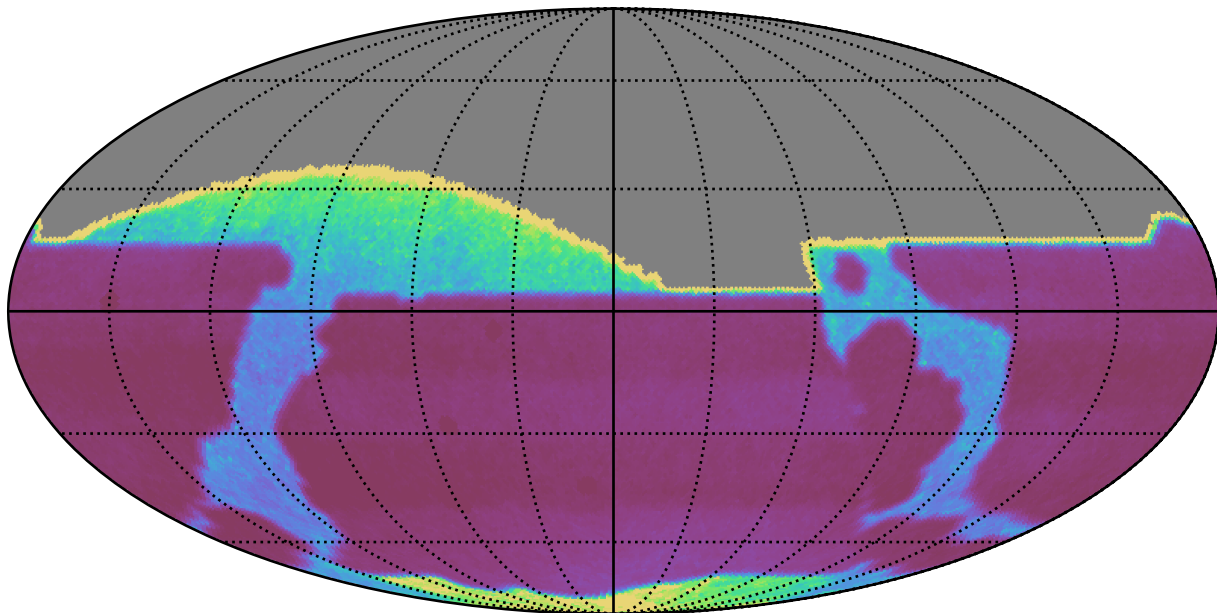
ddf_acor_sf30_lsf40_lsr50_v3.4_10yrs : properMotion
