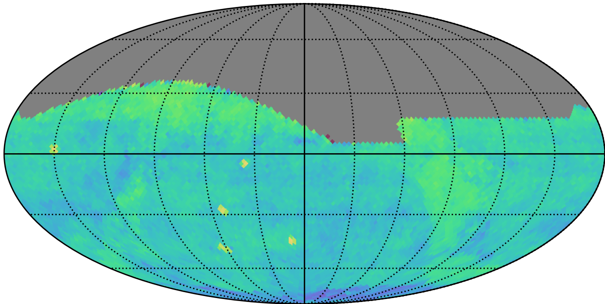
ddf_acor_sf30_lsf40_lsr50_v3.4_10yrs (g or r or i): PairFraction
