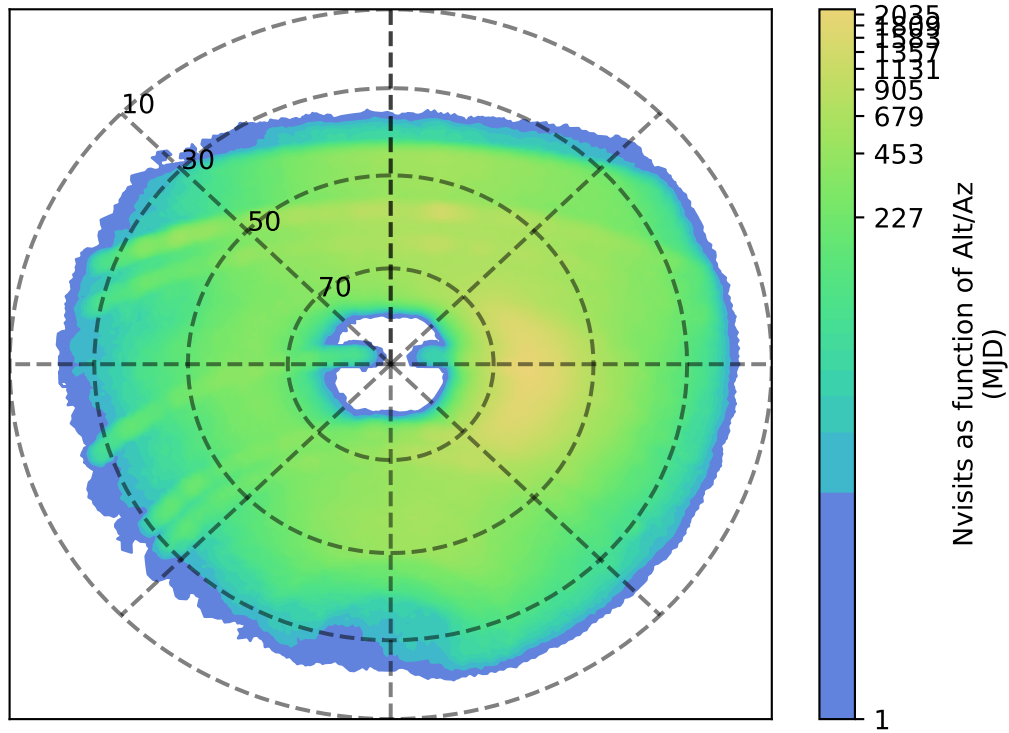
ddf_acor_sf30_lsf40_lsr50_v3.4_10yrs y: Nvisits as function of Alt/Az
