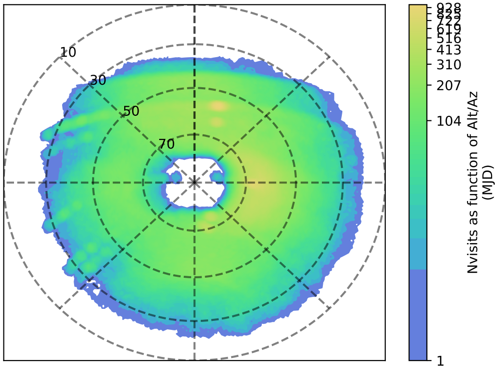
ddf_acor_sf30_lsf40_lsr50_v3.4_10yrs u: Nvisits as function of Alt/Az
