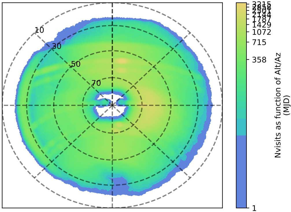
ddf_acor_sf30_lsf40_lsr50_v3.4_10yrs r: Nvisits as function of Alt/Az
