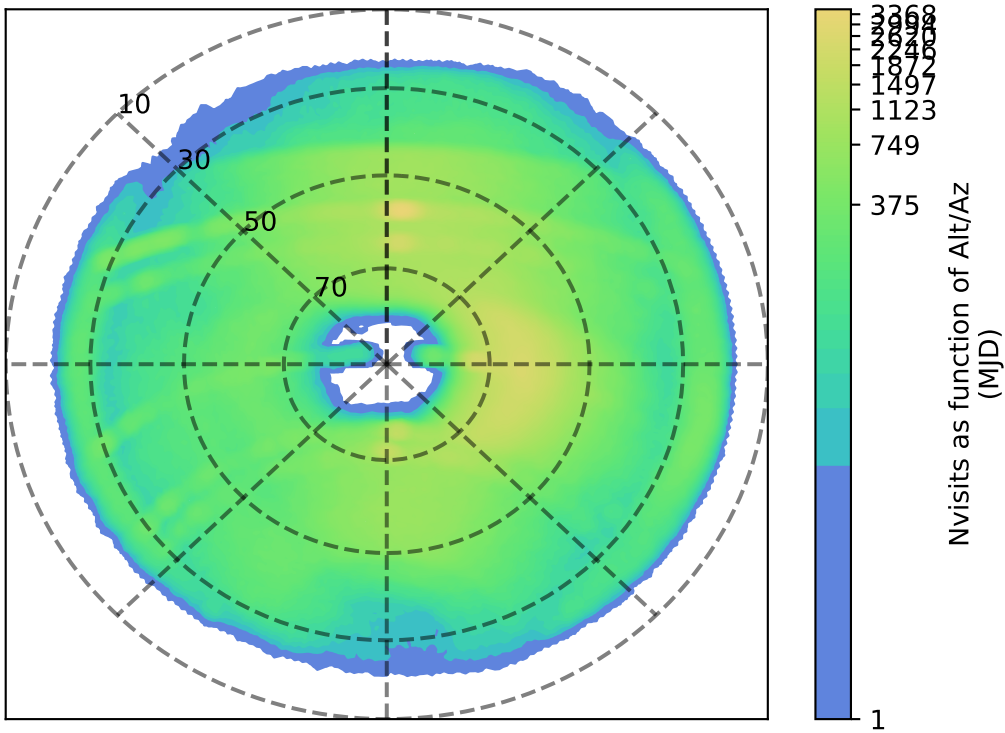
ddf_acor_sf30_lsf40_lsr50_v3.4_10yrs i: Nvisits as function of Alt/Az
