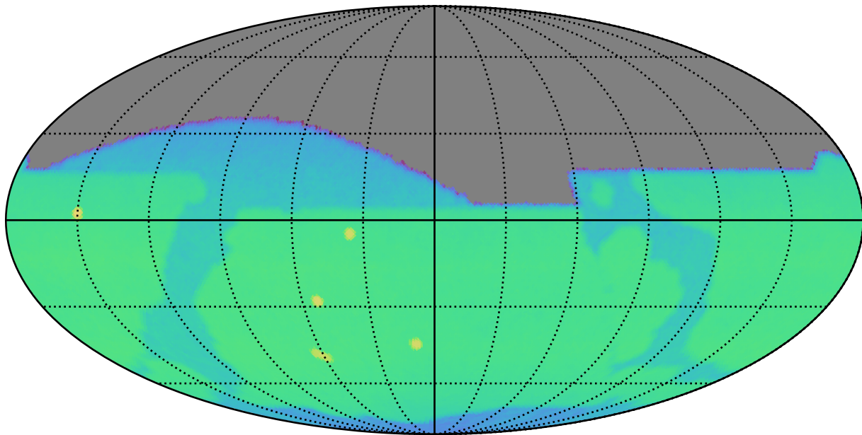
ddf_acor_sf30_lsf40_lsr50_v3.4_10yrs i: CoaddM5
