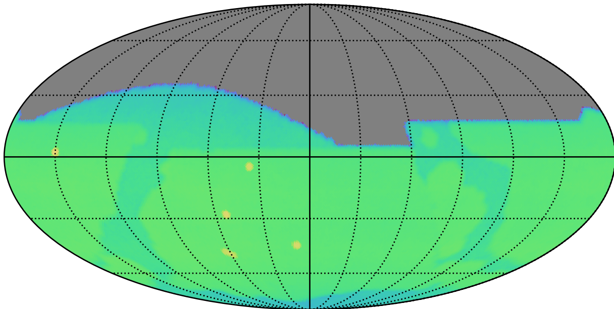
ddf_acor_sf30_lsf40_lsr50_v3.4_10yrs : CoaddM5
