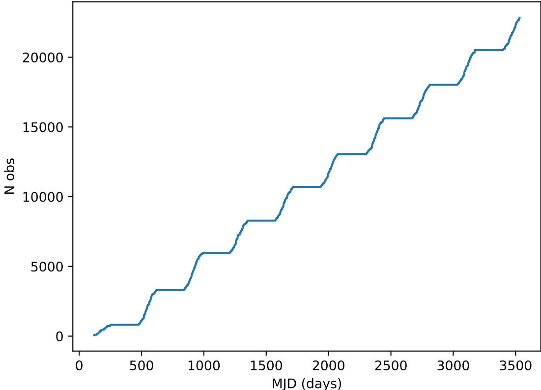
ddf_acor_sf30_lsf40_lsr50_v3.4_10yrs all bands: DD:XMM_LSS Cumulative NVisits
