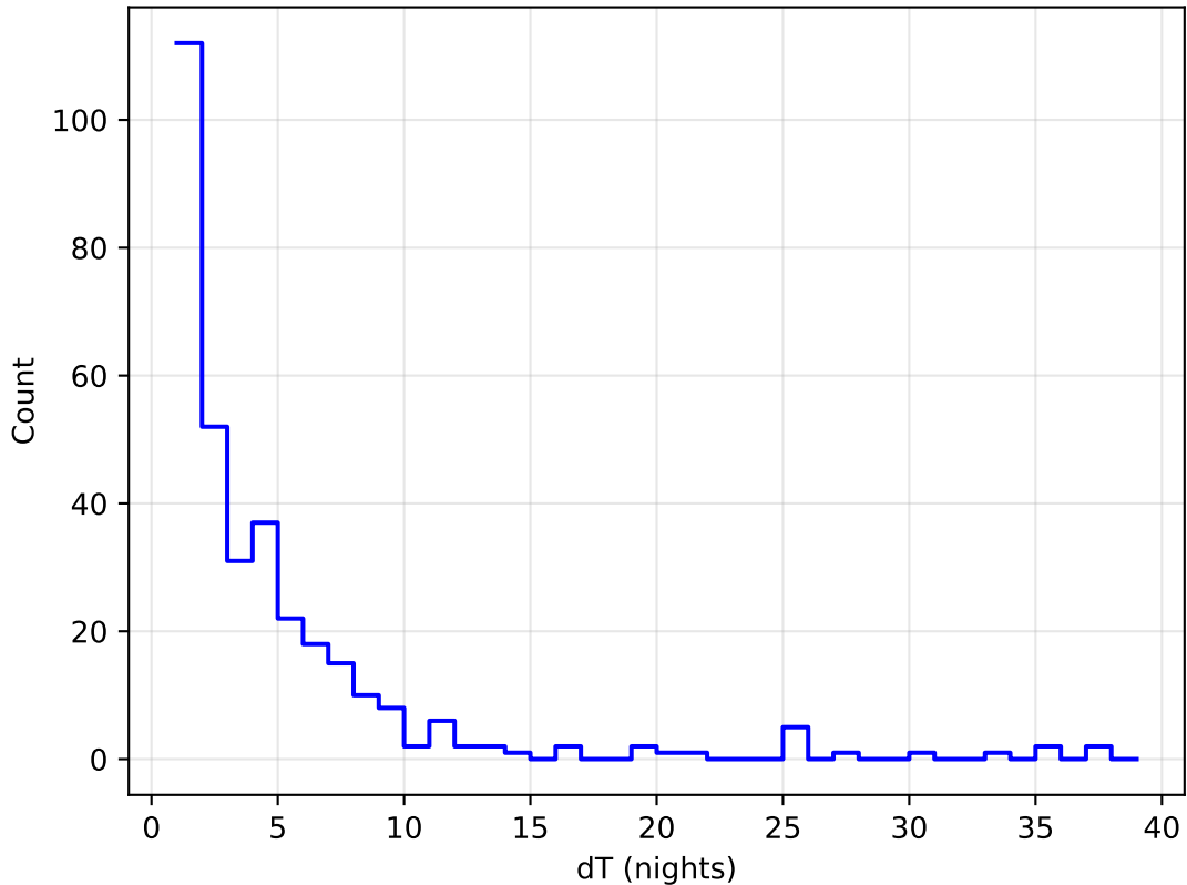
ddf_acor_sf30_lsf40_lsr50_v3.4_10yrs all bands: DD:WFD Delta Nights Histogram
