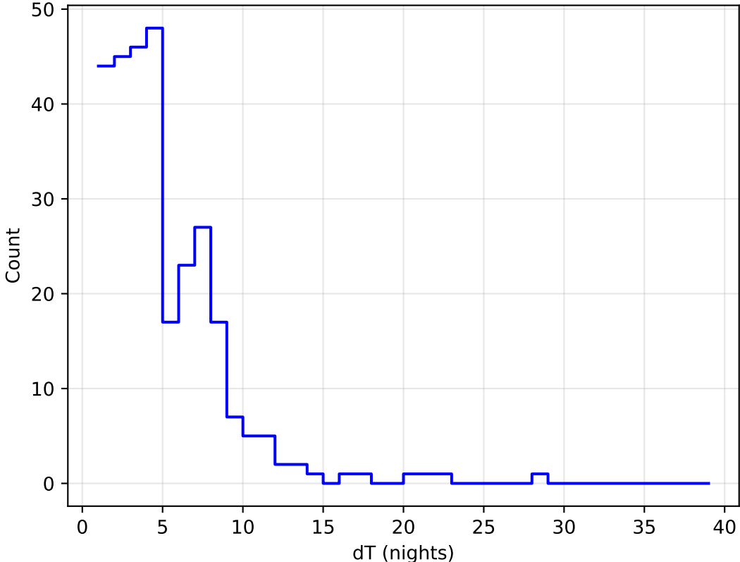
ddf_acor_sf30_lsf40_lsr50_v3.4_10yrs all bands: DD:EDFS Delta Nights Histogram
