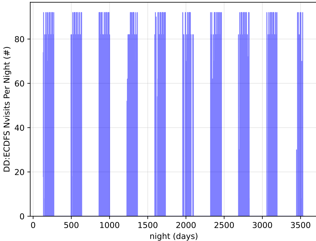
ddf_acor_sf30_lsf40_lsr50_v3.4_10yrs all bands: DD:ECDFS Nvisits Per Night
