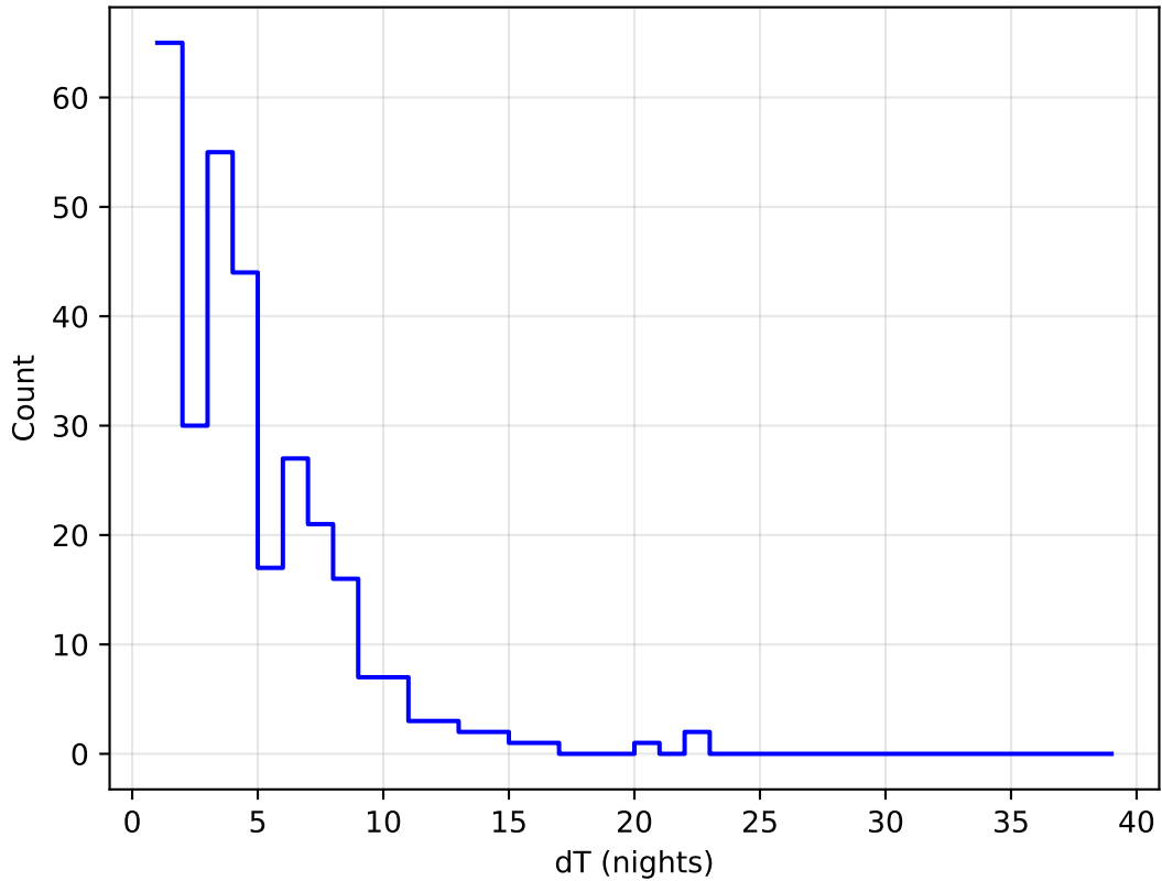
ddf_acor_sf30_lsf40_lsr50_v3.4_10yrs all bands: DD:ECDFS Delta Nights Histogram
