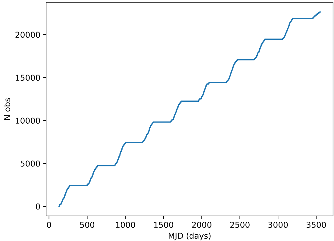
ddf_acor_sf30_lsf40_lsr50_v3.4_10yrs all bands: DD:ECDFS Cumulative NVisits
