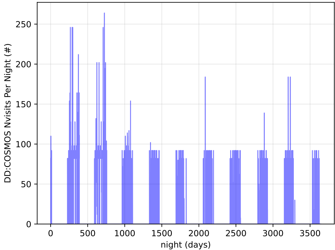
ddf_acor_sf30_lsf40_lsr50_v3.4_10yrs all bands: DD: COSMOS Nvisits Per Night
