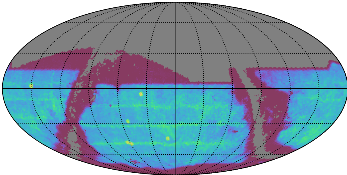
ddf_acor_sf30_lsf40_lsr20_v3.4_10yrs : SNSLMetric
