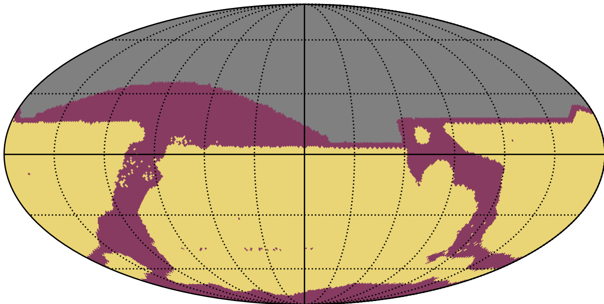
ddf_acor_sf30_lsf40_lsr20_v3.4_10yrs : RapidRevisits
