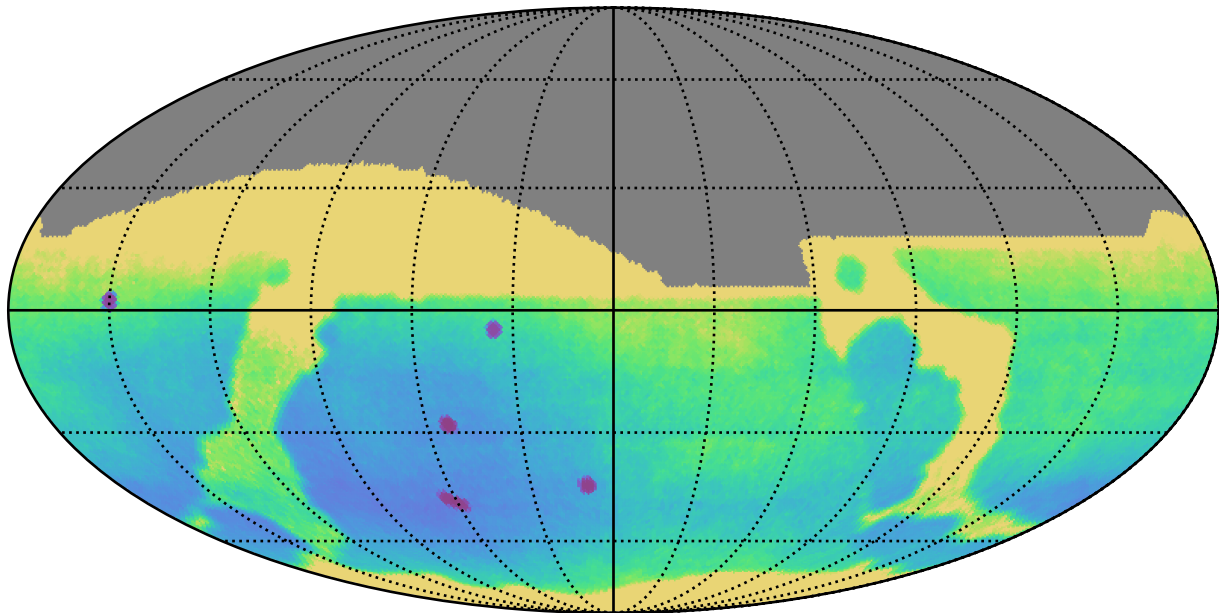
ddf_acor_sf30_lsf40_lsr20_v3.4_10yrs : Parallax Uncert @ 24.0
