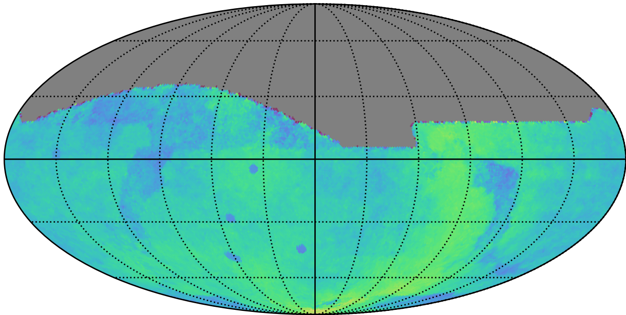
ddf_acor_sf30_lsf40_lsr20_v3.4_10yrs : Parallax Coverage @ 24.0
