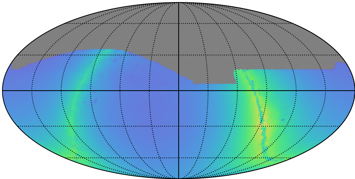
ddf_acor_sf30_lsf40_lsr20_v3.4_10yrs r: Nstars_no_crowding
