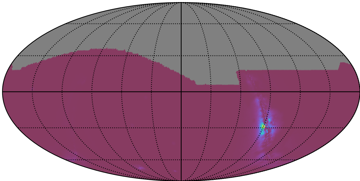
ddf_acor_sf30_lsf40_lsr20_v3.4_10yrs : NlcPoints
