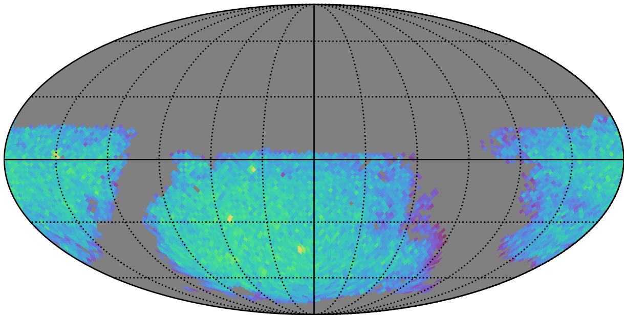
ddf_acor_sf30_lsf40_lsr20_v3.4_10yrs gi: LVDwarfs
