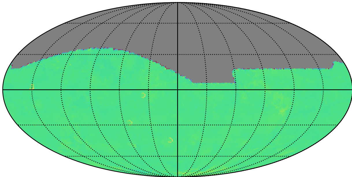
ddf_acor_sf30_lsf40_lsr20_v3.4_10yrs r: Kuiper rotTelPos
