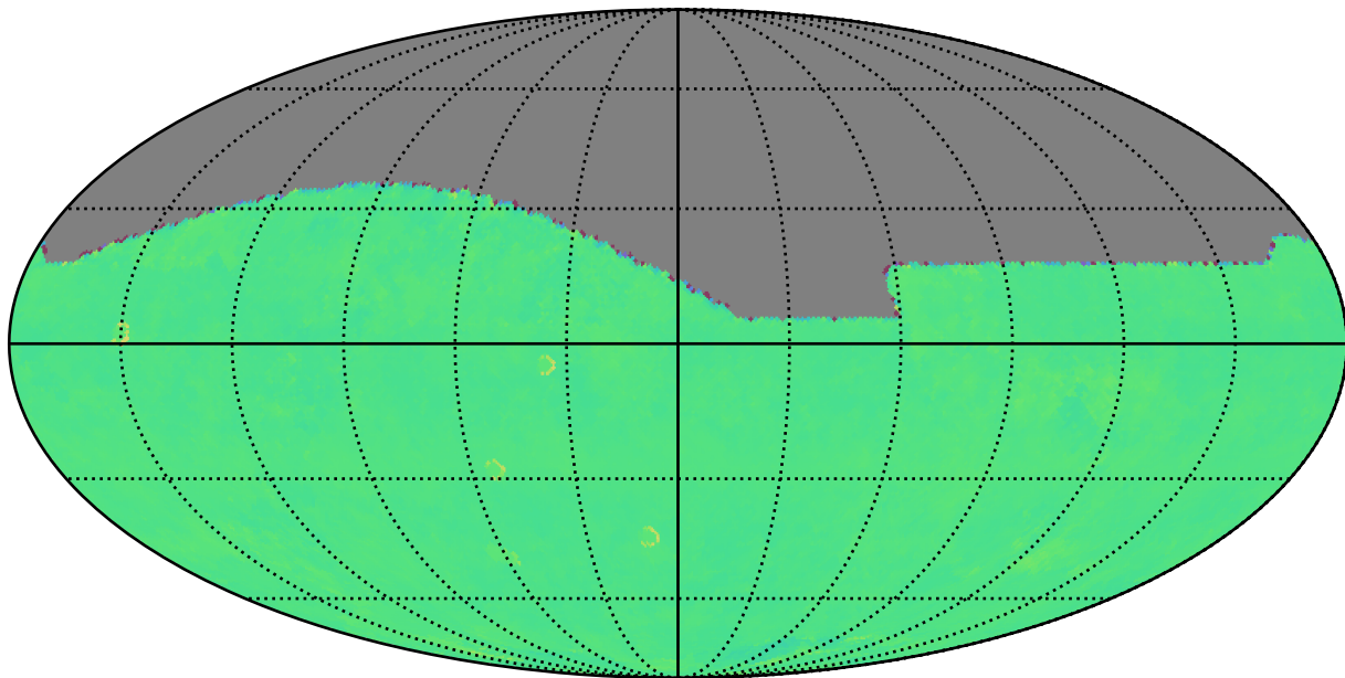
ddf_acor_sf30_lsf40_lsr20_v3.4_10yrs i: Kuiper rotTelPos
