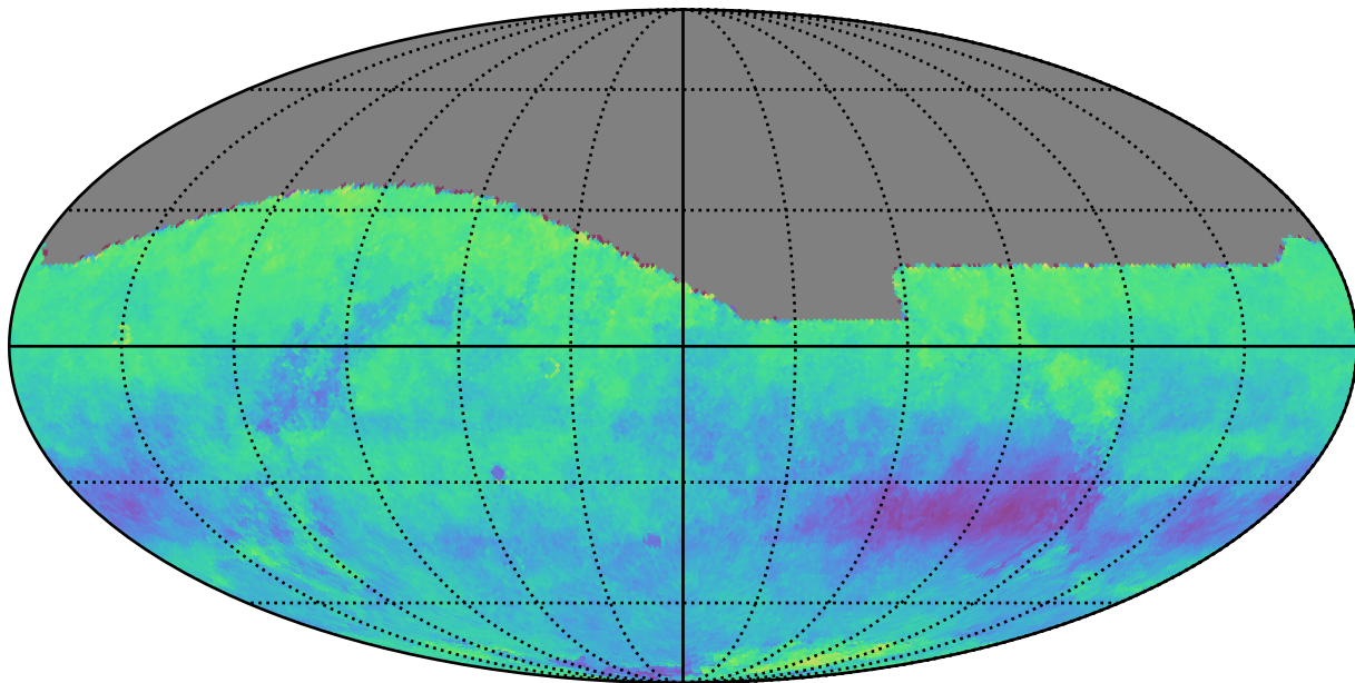
ddf_acor_sf30_lsf40_lsr20_v3.4_10yrs r: Kuiper rotSkyPos
