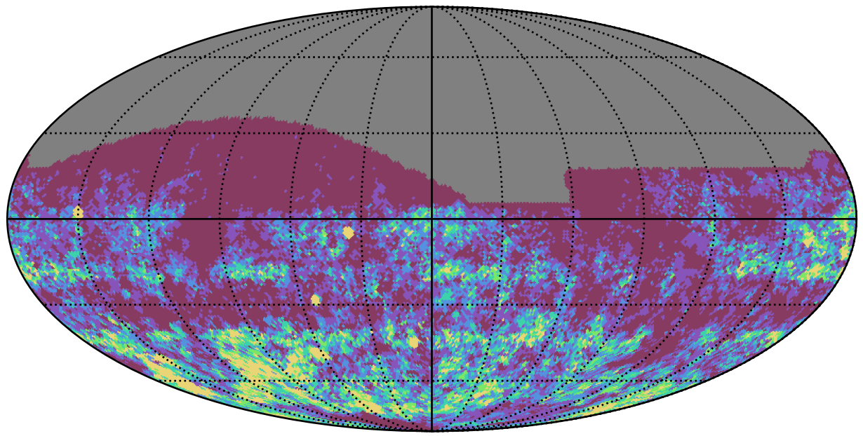
ddf_acor_sf30_lsf40_lsr20_v3.4_10yrs r band: Gaps_3hr
