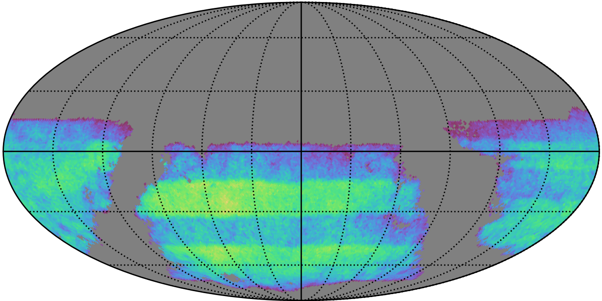
ddf_acor_sf30_lsf40_lsr20_v3.4_10yrs i band non-DD year 3: Exgalml5WithCuts
