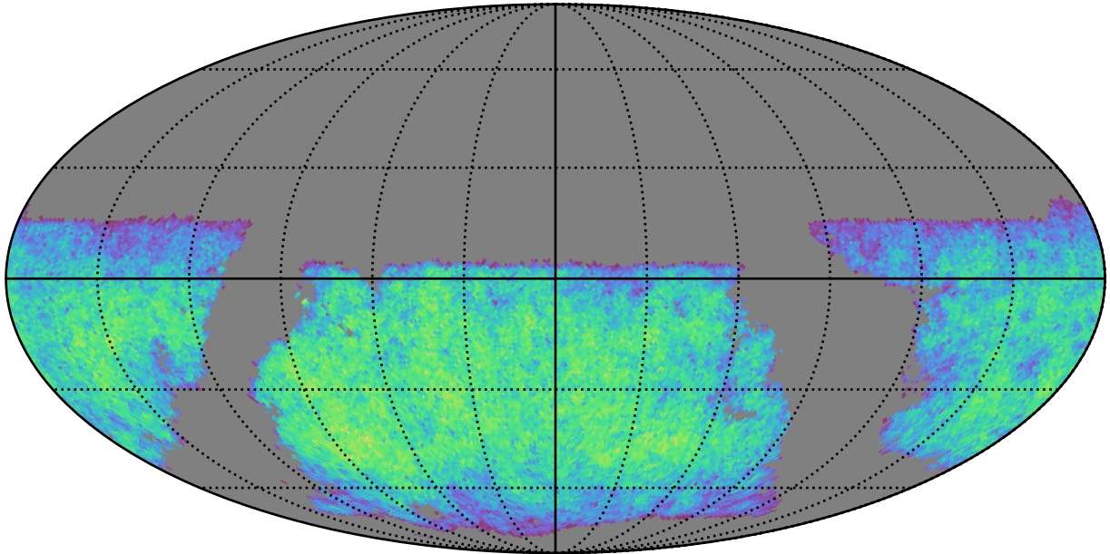
ddf_acor_sf30_lsf40_lsr20_v3.4_10yrs i band non-DD year 1: ExgalM5WithCuts
