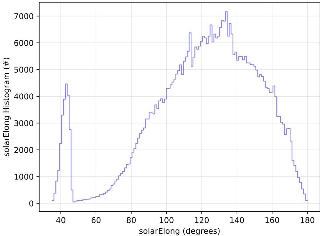
ddf_acor_sf30_lsf40_lsr20_v3.4_10yrs WFD z band: solarElong Histogram
