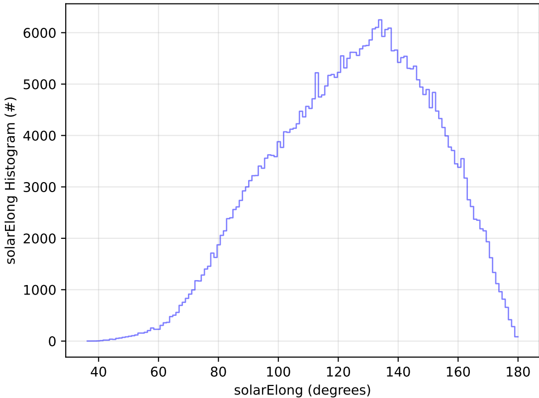
ddf_acor_sf30_lsf40_lsr20_v3.4_10yrs WFD y band: solarElong Histogram
