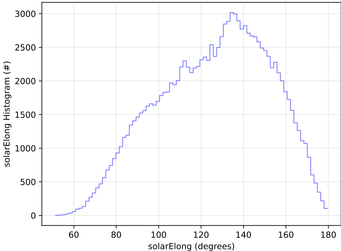
ddf_acor_sf30_lsf40_lsr20_v3.4_10yrs WFD u band: solarElong Histogram
