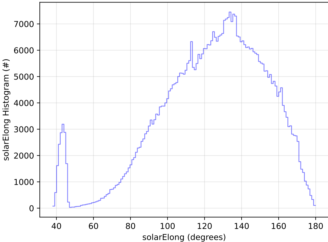
ddf_acor_sf30_lsf40_lsr20_v3.4_10yrs WFD r band: solarElong Histogram
