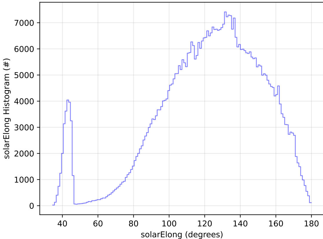
ddf_acor_sf30_lsf40_lsr20_v3.4_10yrs WFD i band: solarElong Histogram
