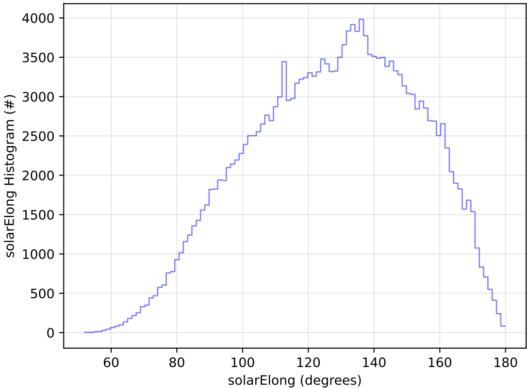
ddf_acor_sf30_lsf40_lsr20_v3.4_10yrs WFD g band: solarElong Histogram
