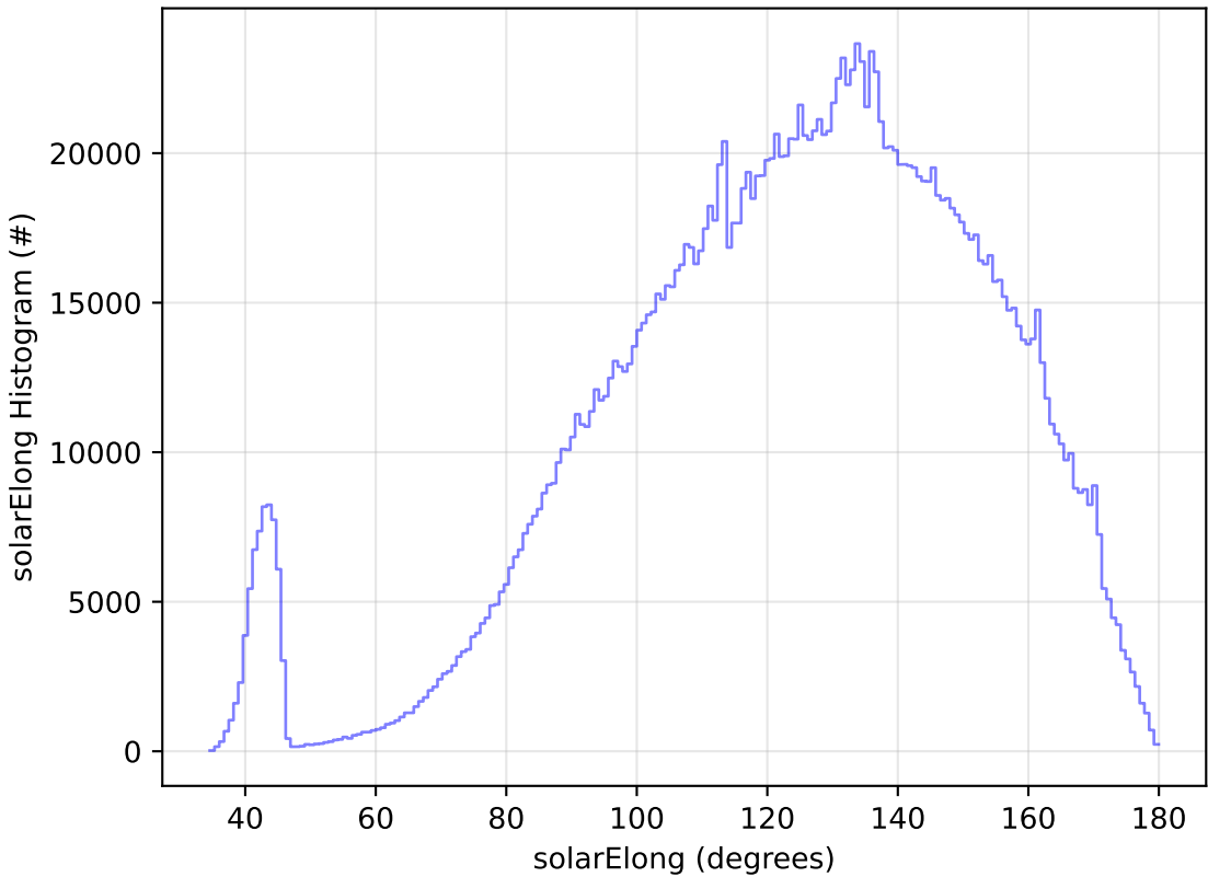
ddf_acor_sf30_lsf40_lsr20_v3.4_10yrs WFD all bands: solarElong Histogram
