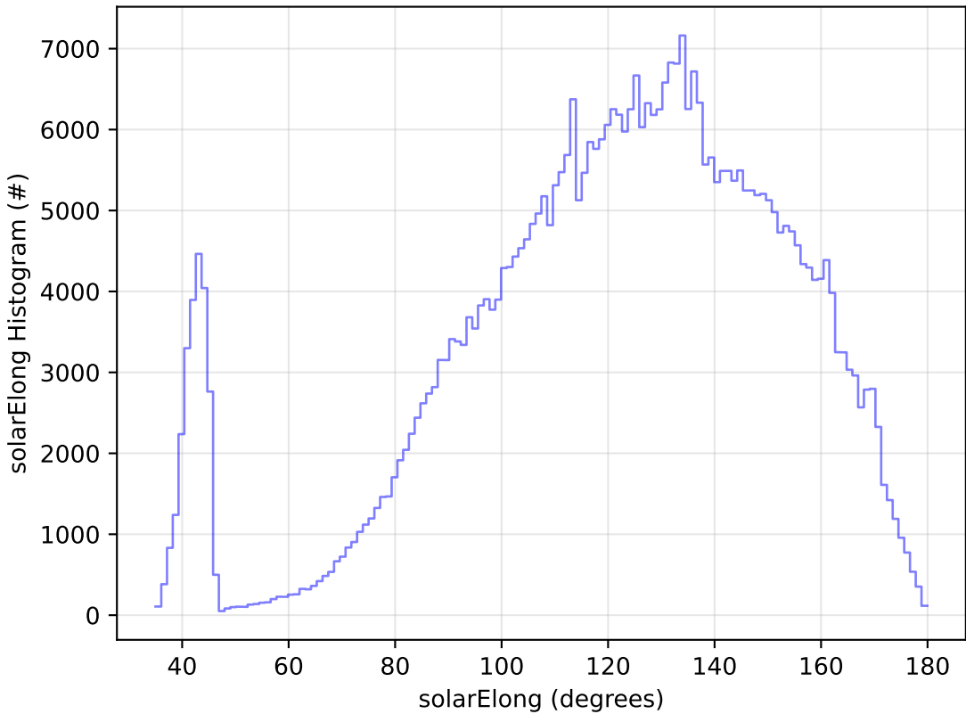
ddf_acor_sf30_lsf40_lsr20_v3.4_10yrs All sky z band: solarElong Histogram
