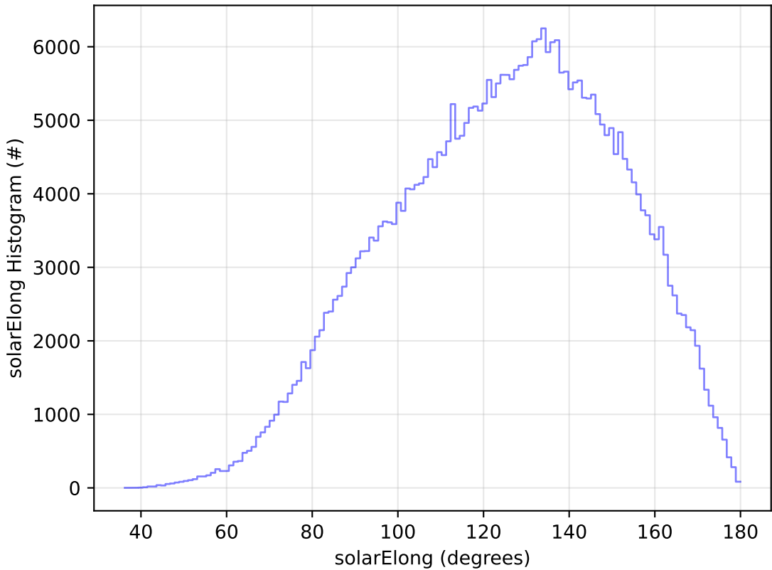
ddf_acor_sf30_lsf40_lsr20_v3.4_10yrs All sky y band: solarElong Histogram
