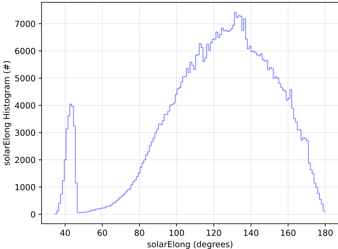
ddf_acor_sf30_lsf40_lsr20_v3.4_10yrs All sky i band: solarElong Histogram
