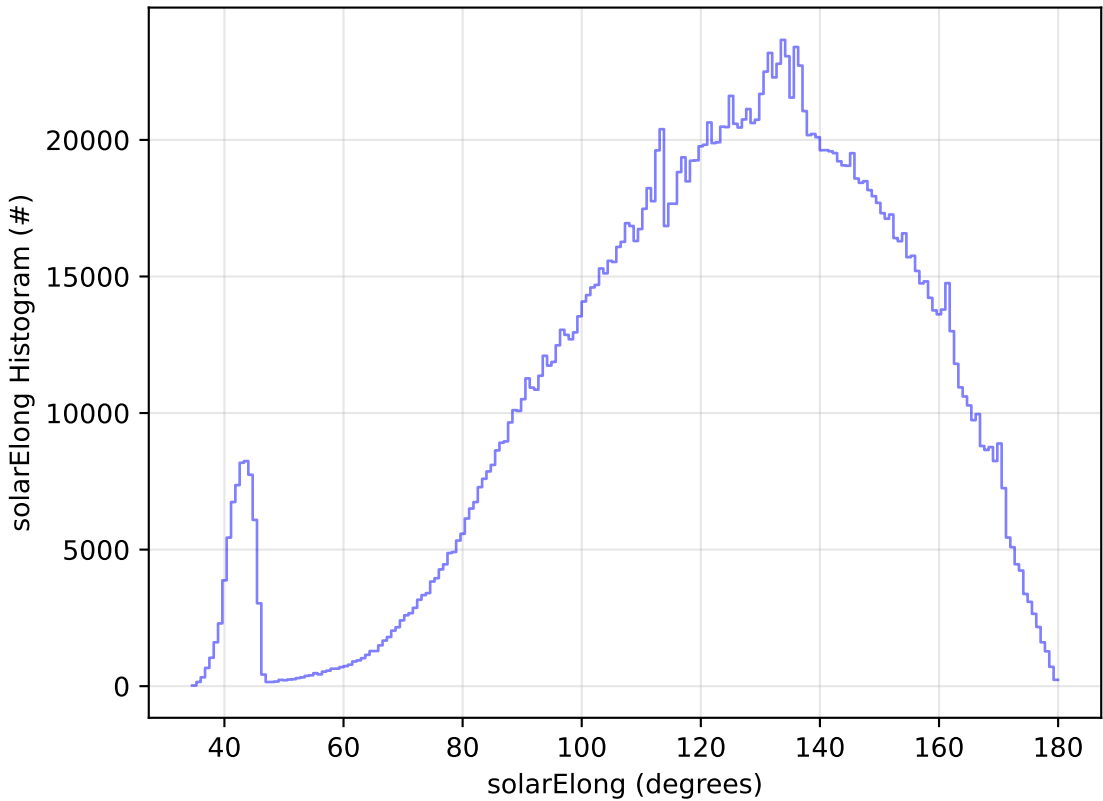
ddf_acor_sf30_lsf40_lsr20_v3.4_10yrs All sky all bands: solarElong Histogram
