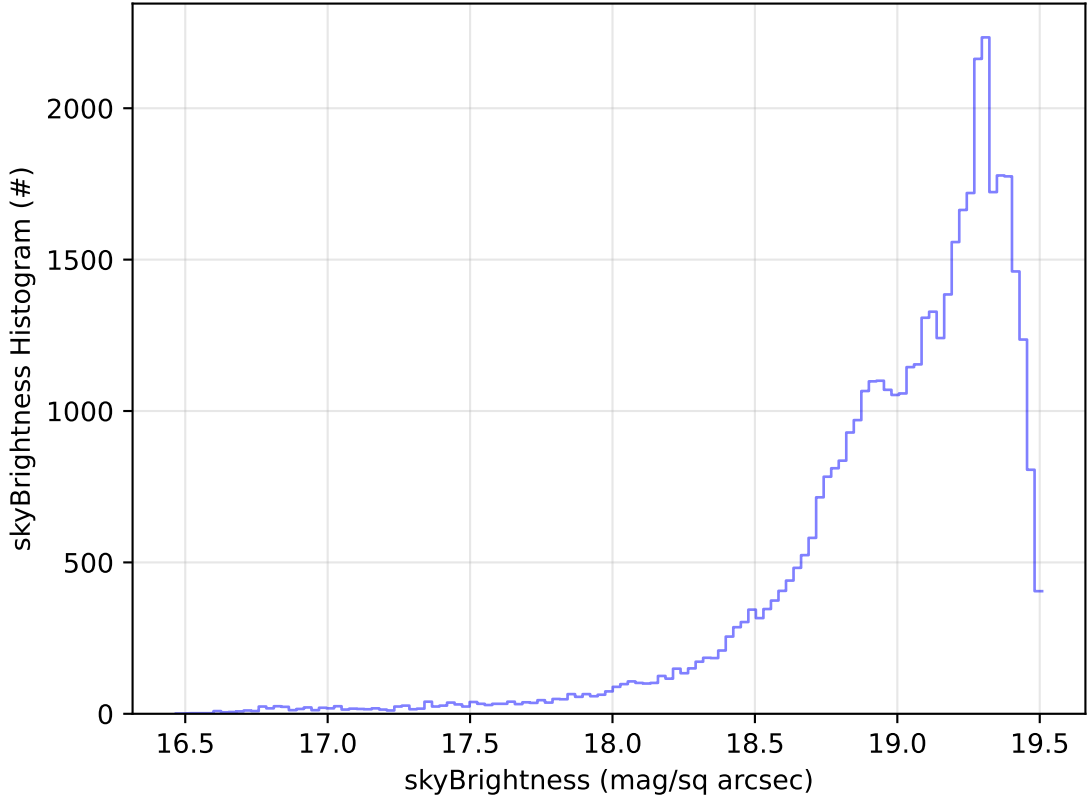
ddf_acor_sf30_lsf40_lsr20_v3.4_10yrs Yr 1 z band: skyBrightness Histogram
