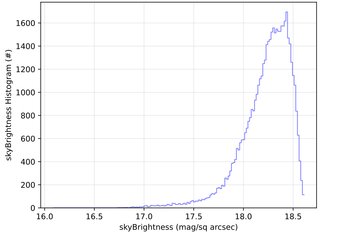
ddf_acor_sf30_lsf40_lsr20_v3.4_10yrs Yr 1 y band: skyBrightness Histogram
