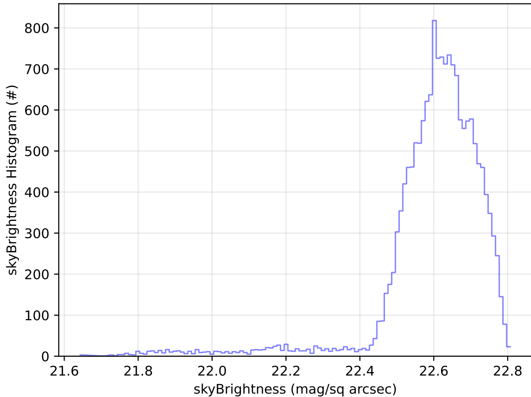
ddf_acor_sf30_lsf40_lsr20_v3.4_10yrs Yr 1 u band: skyBrightness Histogram
