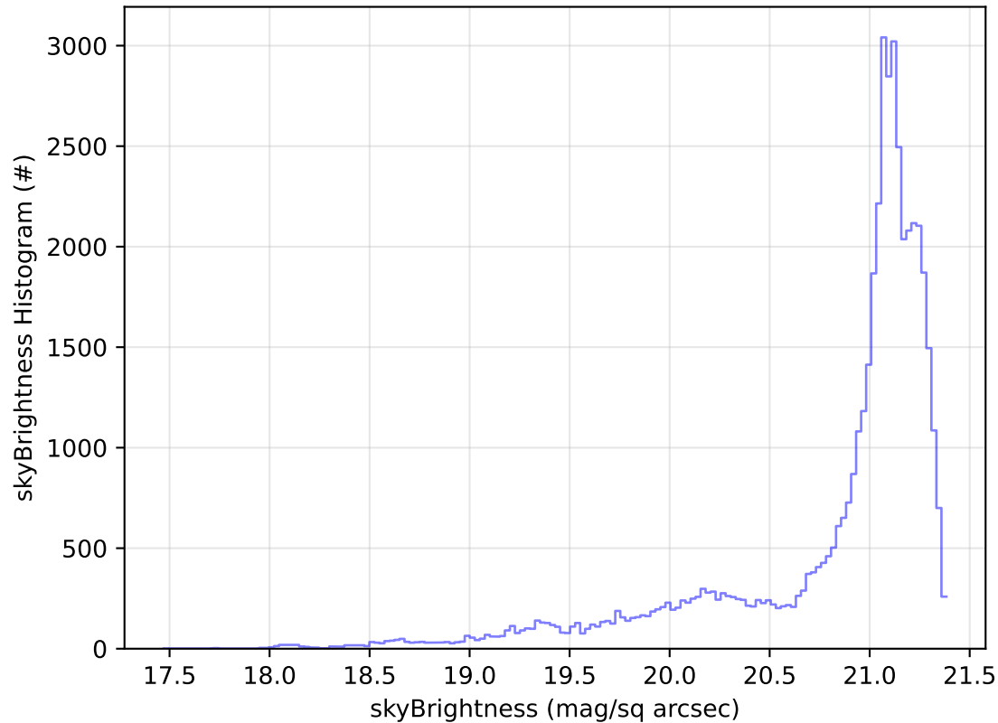
ddf_acor_sf30_lsf40_lsr20_v3.4_10yrs Yr 1 r band: skyBrightness Histogram
