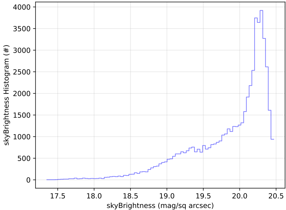
ddf_acor_sf30_lsf40_lsr20_v3.4_10yrs Yr 1 i band: skyBrightness Histogram
