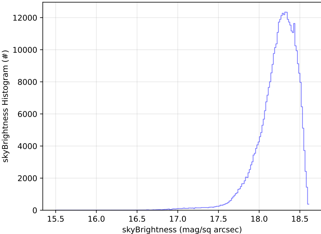
ddf_acor_sf30_lsf40_lsr20_v3.4_10yrs WFD y band: skyBrightness Histogram
