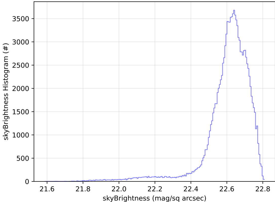
ddf_acor_sf30_lsf40_lsr20_v3.4_10yrs WFD u band: skyBrightness Histogram
