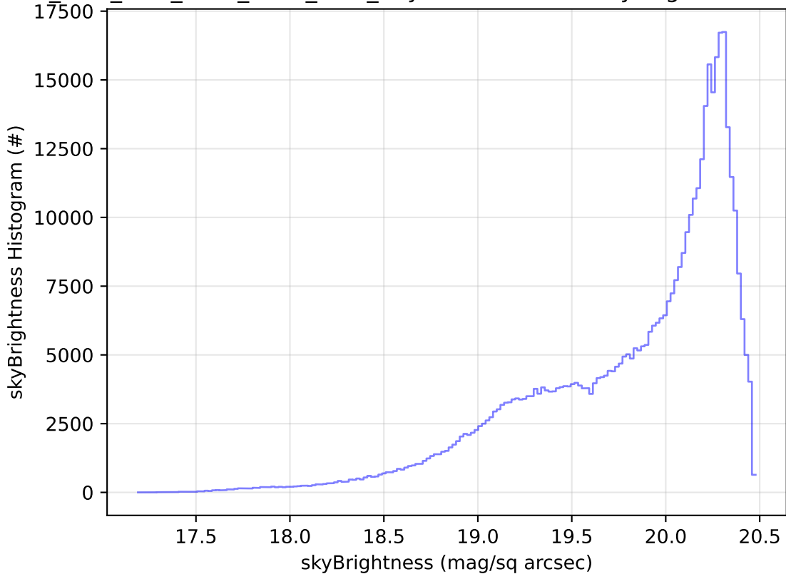
ddf_acor_sf30_lsf40_lsr20_v3.4_10yrs WFD i band: skyBrightness Histogram
