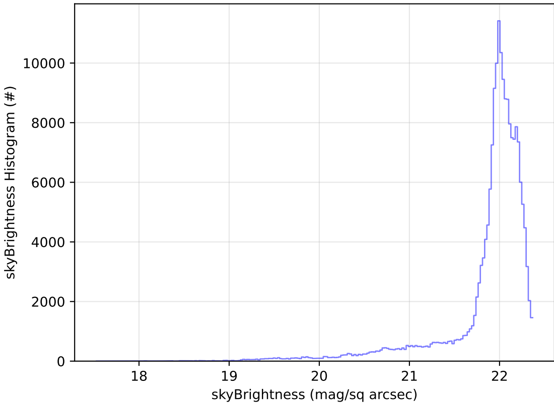
ddf_acor_sf30_lsf40_lsr20_v3.4_10yrs WFD g band: skyBrightness Histogram
