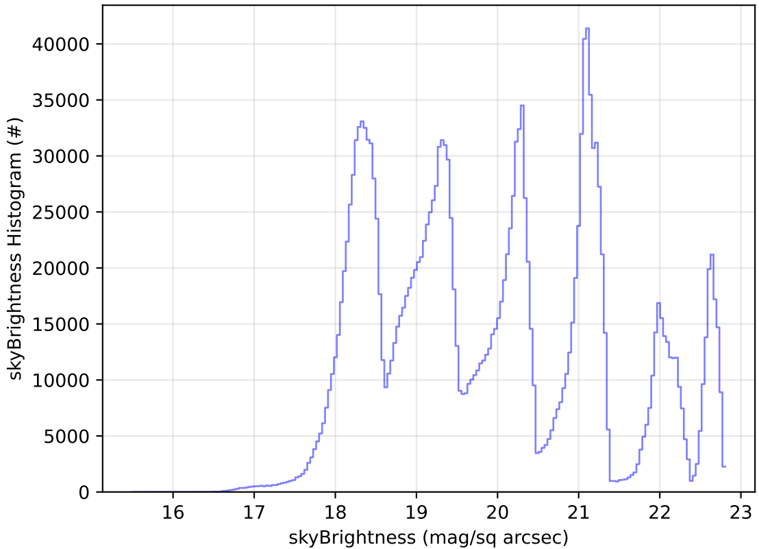
ddf_acor_sf30_lsf40_lsr20_v3.4_10yrs WFD all bands: skyBrightness Histogram
